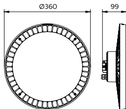
BY698P GreenPerform High-bay gen3
