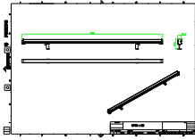
Floodlight surface LED
